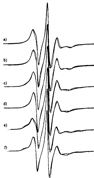
FIGURE 2: Representative ESR spectrum of various spin-labeled lipids in nAChR-rich membranes given in pairs corresponding to controls (a, c, and e) and samples treated with 16.7 mM 1-hexanol (b, d, and f) at 7 °C for the three spin-labels examined: (a and b) 14-PCSL; (c and d) 14-PGSL; (e and f) 14-SASL. The experimental spectra (full lines) are overlaid with the best-fitting simulated (dashed lines) spectra, which have been computed from the exchange-coupled, modified Bloch equations (see Materials and Methods). Total scan width, 10 mT.
