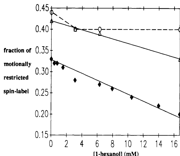
FIGURE 3: Fraction of motionally restricted, spin-labeled lipid determined at various concentrations of added 1-hexanol, as derived from computer simulations of experimental spectra from 14-SASL (○), 14-PCSL (●), and 14-PGSL (△) probing nAChR-enriched membranes at 7 °C.
